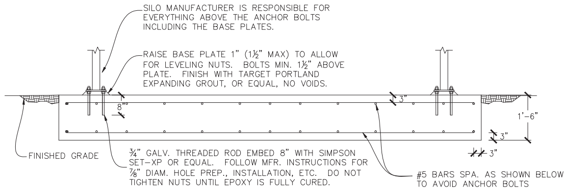
FOUNDATION SECTION (SCALE: 3/4" = 1'-0")
