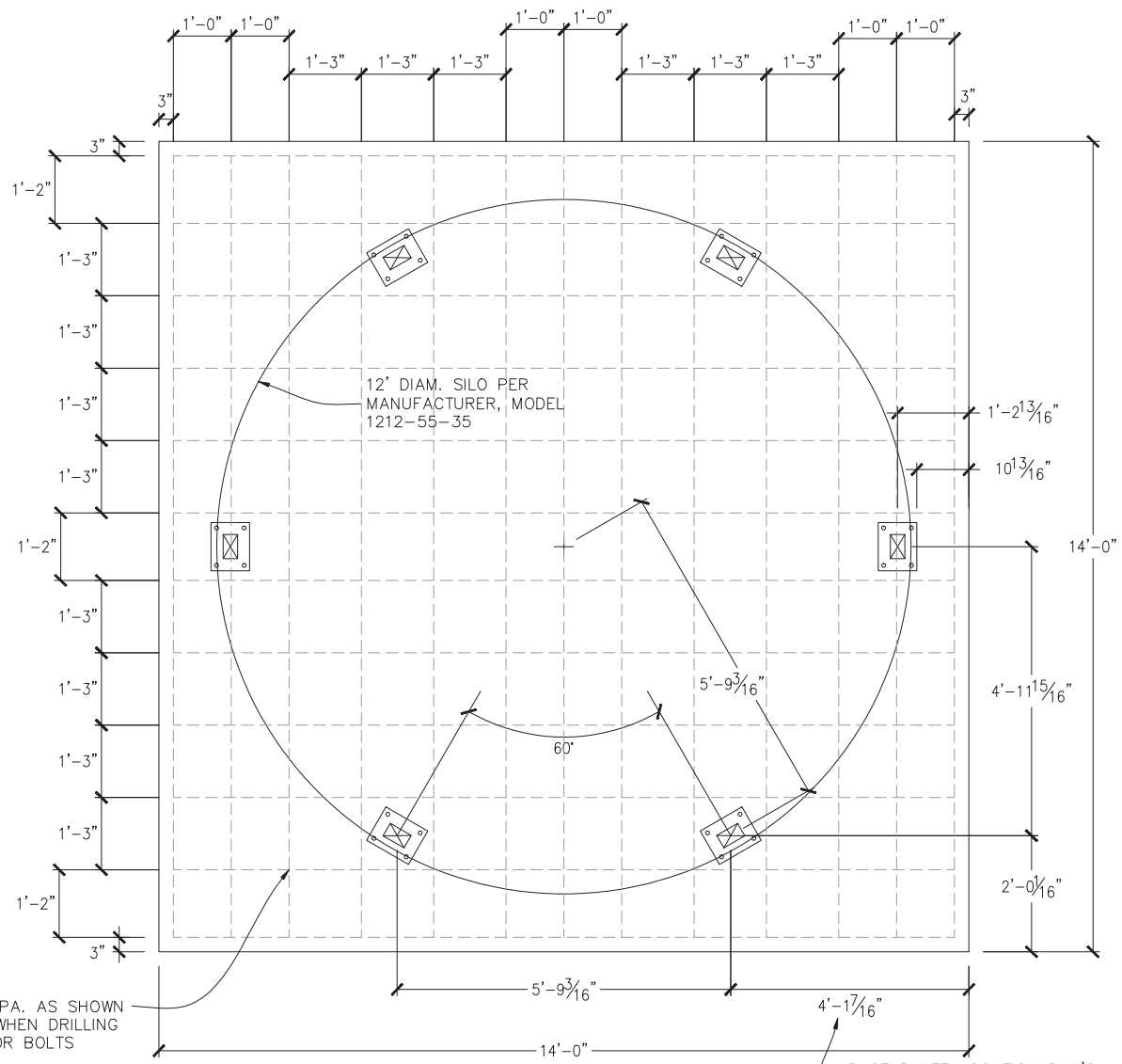
FOUNDATION PLAN (SCALE: 3/4" = 1'-0")
